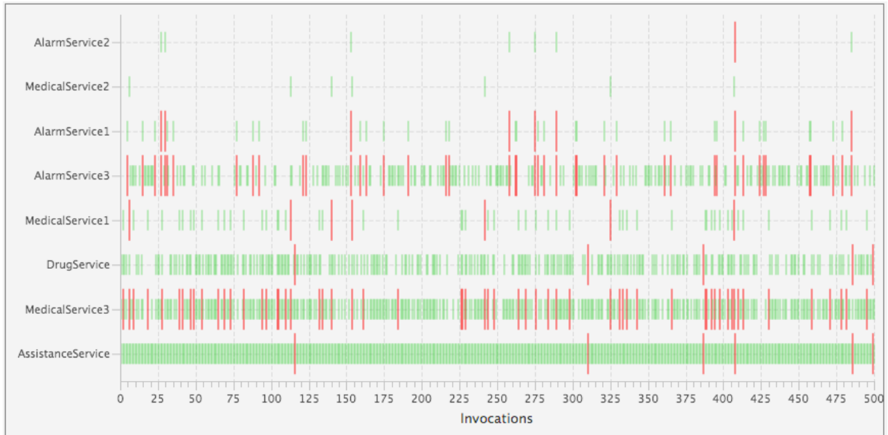
Fig. 4. Reliability graph for the case study; successful service invocations are represented by small vertical lines and failed invocations by larger lines.
